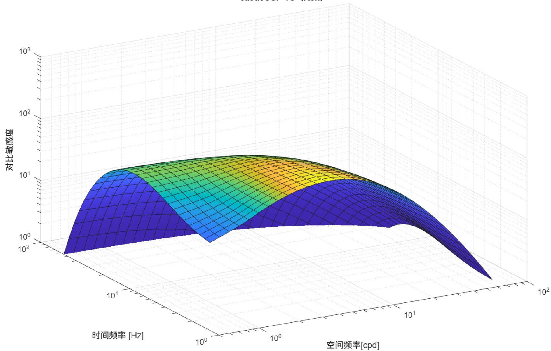
castleCSF-TS (Ach)
